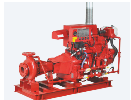
DIESEL ENGINE DRIVEN FIRE PUMP
